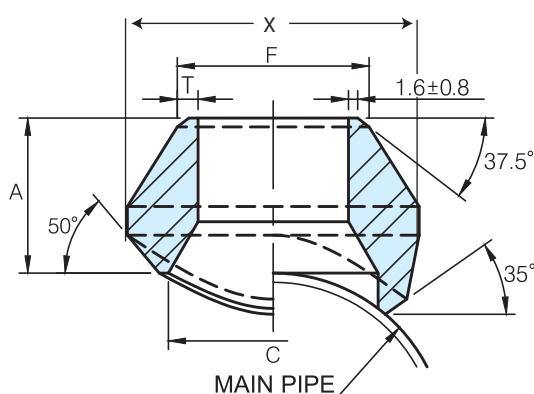
REDUCING WAY
