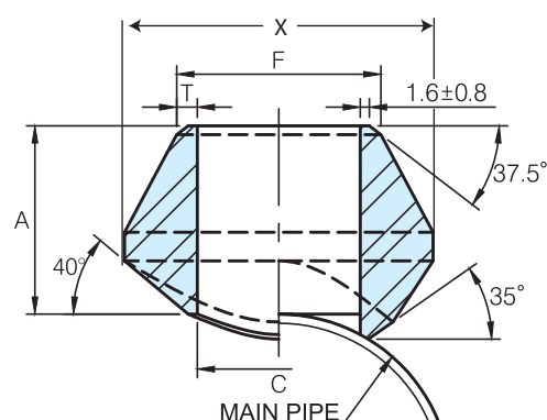
STRAIGHT WAY
