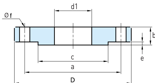
RF
